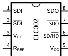
Figure 1. 8-Pin SOIC
